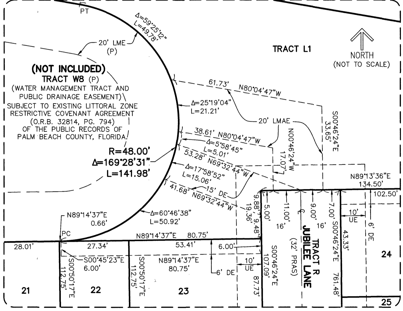
DETAIL "B"
